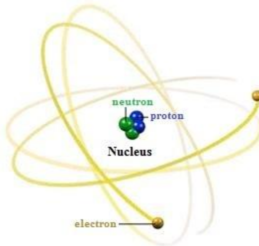
II. 4: Quantum Physic atomic structure
